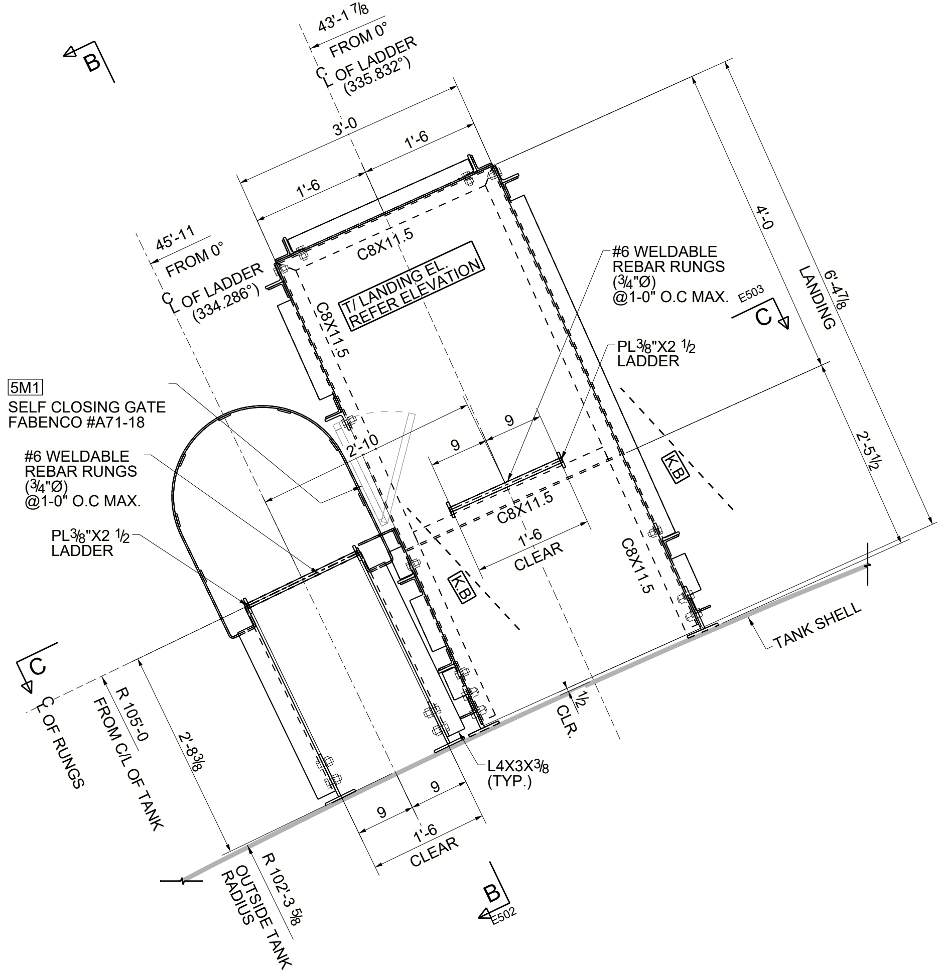
LADDER LOCATION PLAN AT LANDING 02, 04 AND 06 AT EL. 1105'-3 1/4", 1143'-3 1/4 AND 1181'-3 1/4 (REFER: PLAN OF EMERGENCY LADDER /DW-10600-01)
