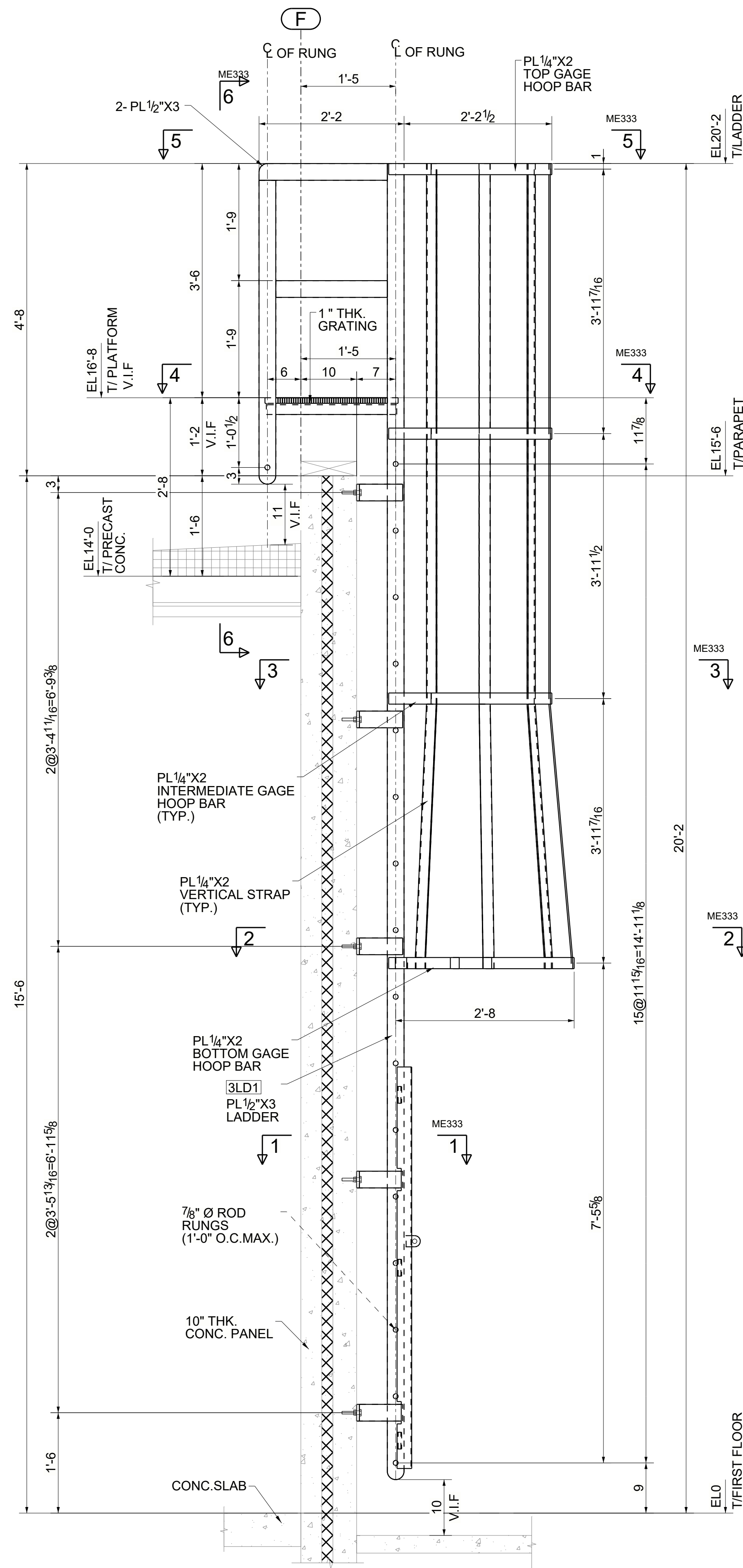
SECTION A - A
