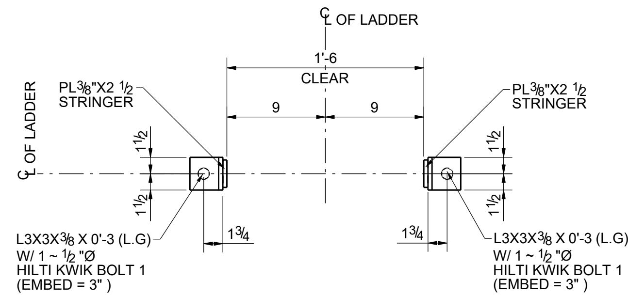
SECTION 5 - 5 33-E3301
