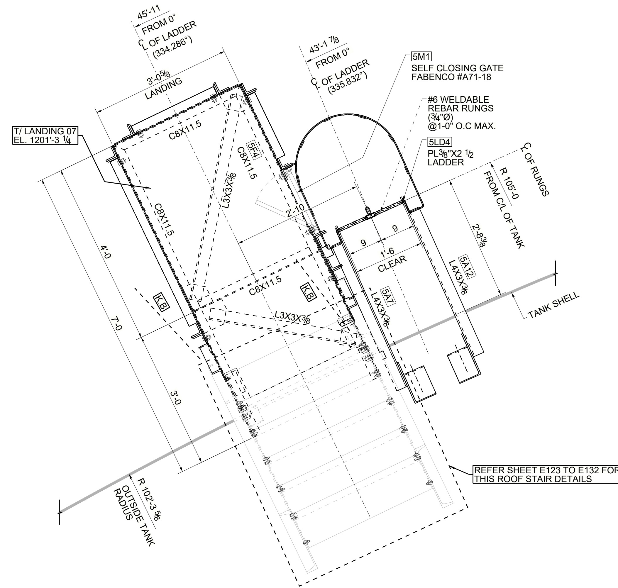
LADDER LOCATION PLAN AT LANDING 07 EL. 1201'-3 1/4 (REFER: PLAN OF EMERGENCY LADDER /DW-10600-01)
