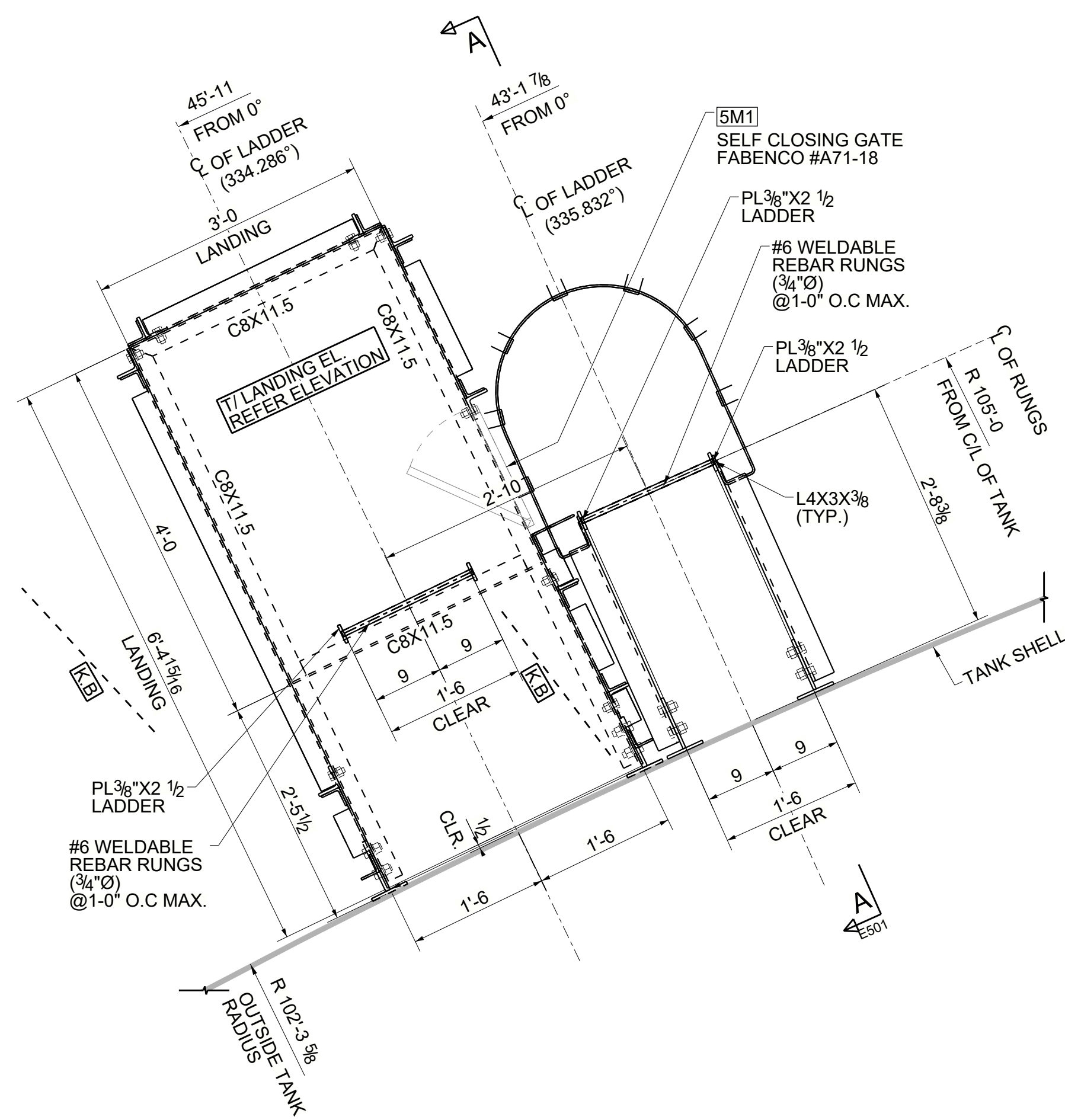
LADDER LOCATION PLAN AT LANDING 01, 03 AND 05 AT EL. 1086'-3 1/4", EL. 1124'-3 1/4 AND EL. 1162'-3 1/4 (REFER: PLAN OF EMERGENCY LADDER /DW-10600-01)
