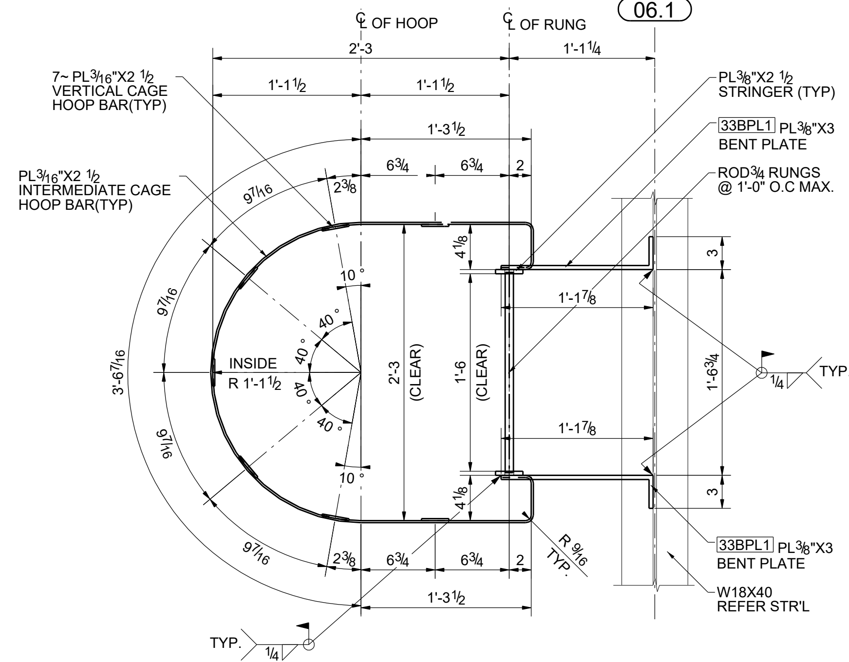
SECTION 2 - 2 33-E3301 INTERMEDIATE CAGE HOOP BAR DETAIL
