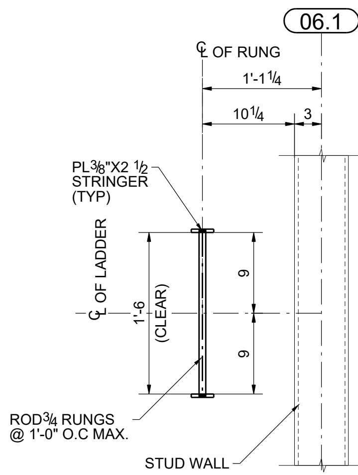
SECTION 4 - 4 33-E3301
