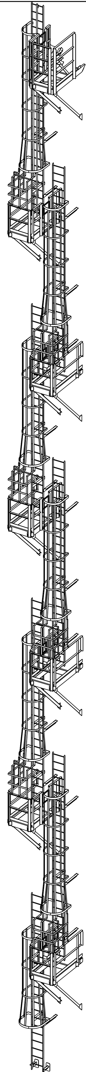
3D VIEW @ EMERGENCY LADDER
