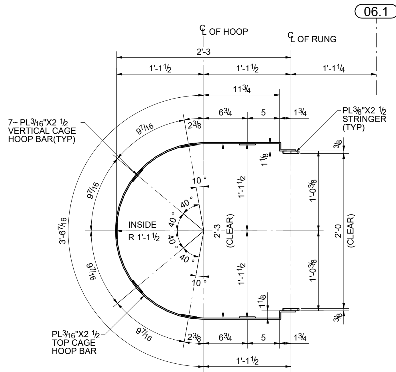
SECTION 1 - 1 33-E3301 TOP CAGE HOOP BAR DETAIL
