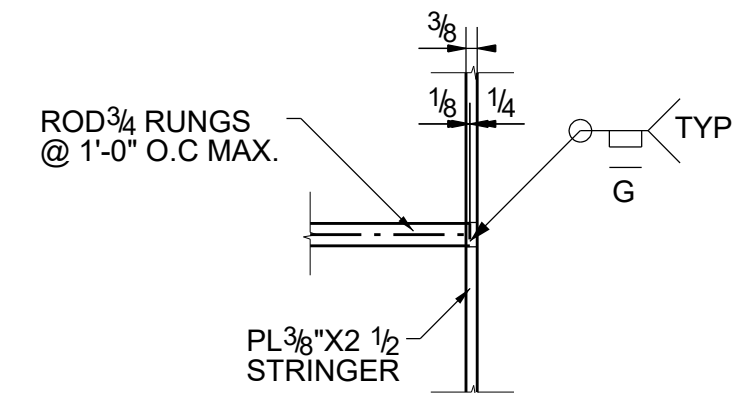
TYPICAL ROD RUNG CONNETION DETAIL
